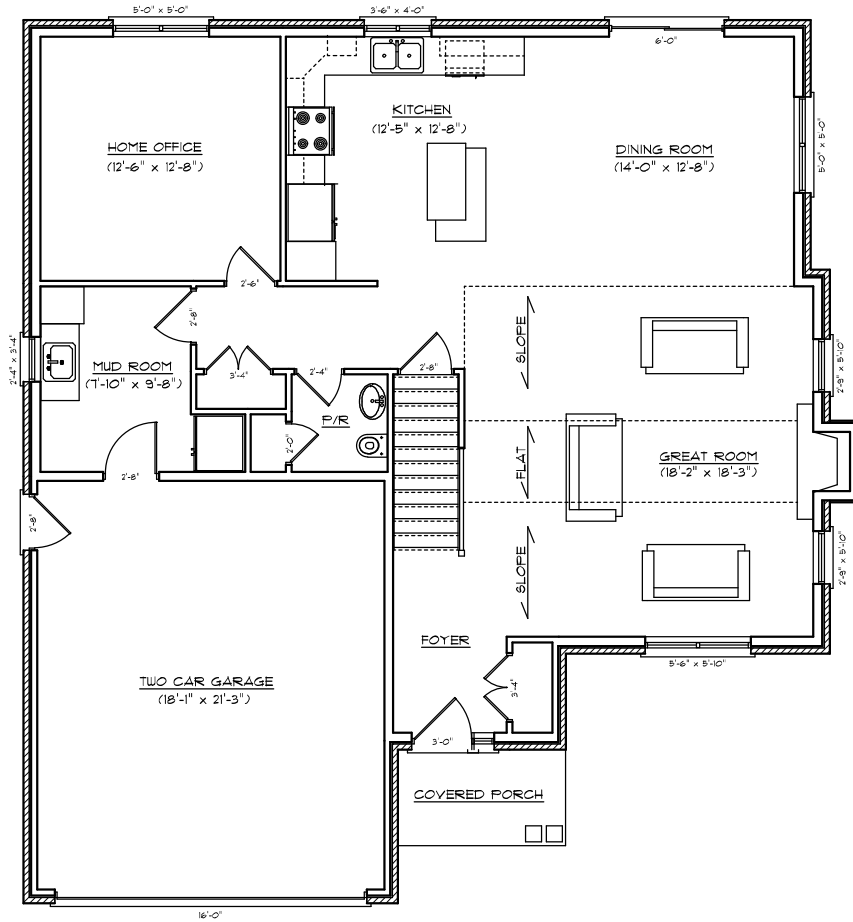
MAIN FLOOR PLAN (APPROX. 1254 SQ. FT.)
