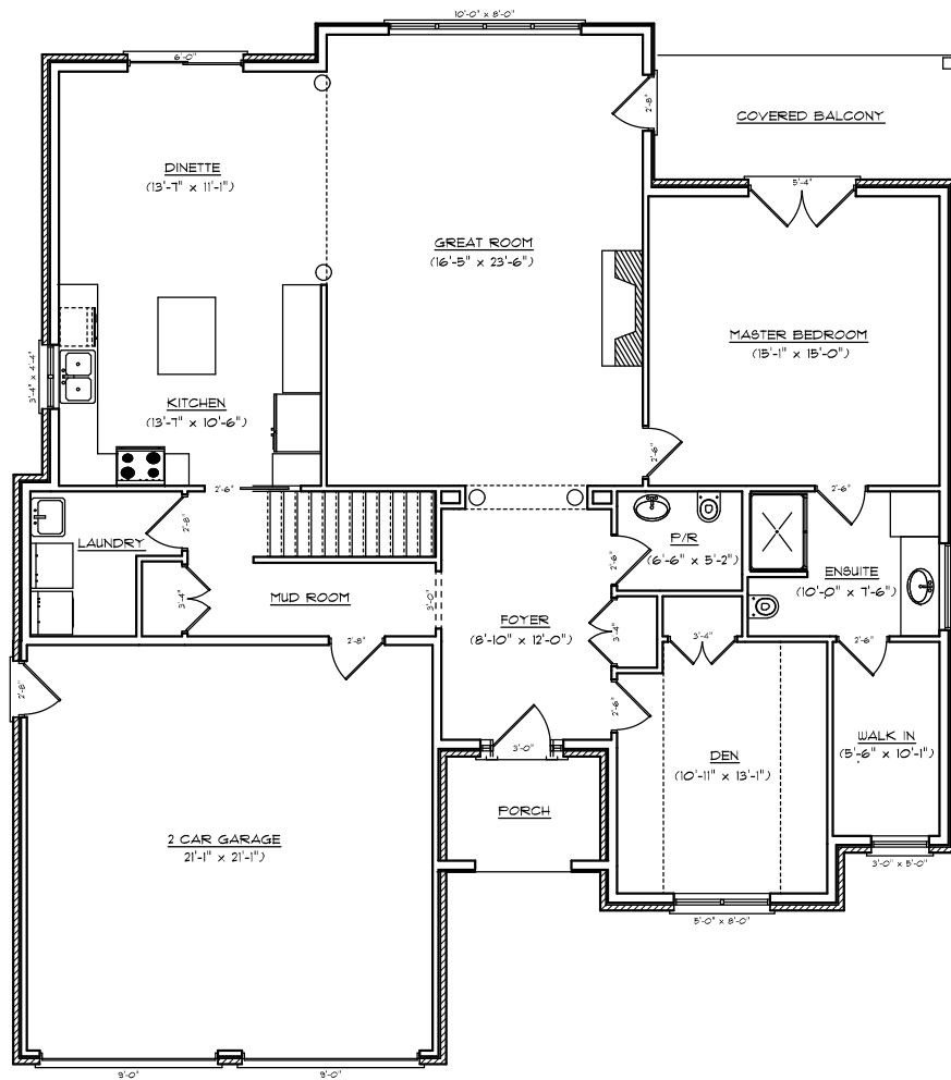
MAIN FLOOR PLAN (APPROX. 1698 SQ. FT.)
