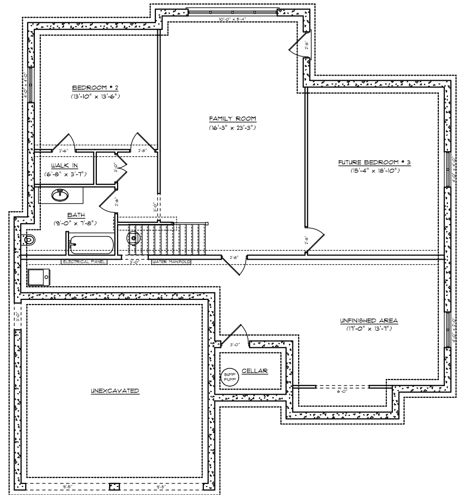
FOUNDATION PLAN (APPROX. 876 SQ. FT.)
