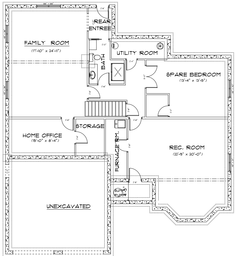
BASEMENT LAYOUT
