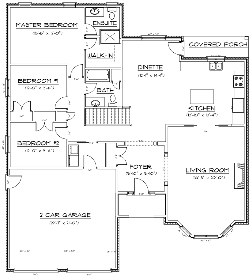
MAIN FLOOR PLAN (APPROX. 1850 SQ)
