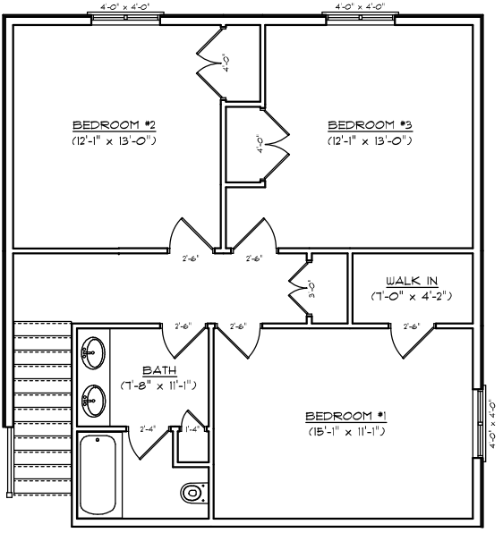
SECOND FLOOR PLAN (APPROX. 786 SQ. FT.)
